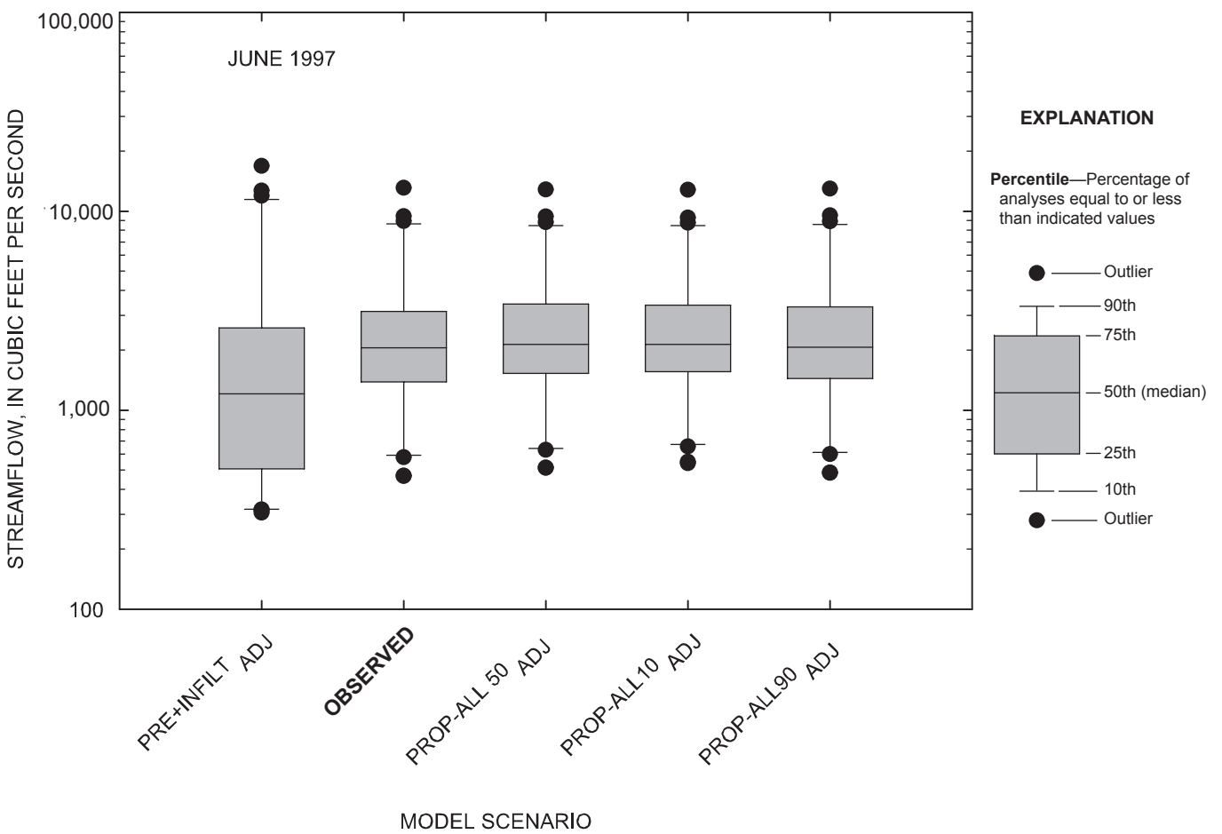
Figure 4-33. Comparison of daily streamflow for observed and simulated conditions at the Marais des Cygnes River near the Kansas-Missouri state line, Kansas, June 1997.
