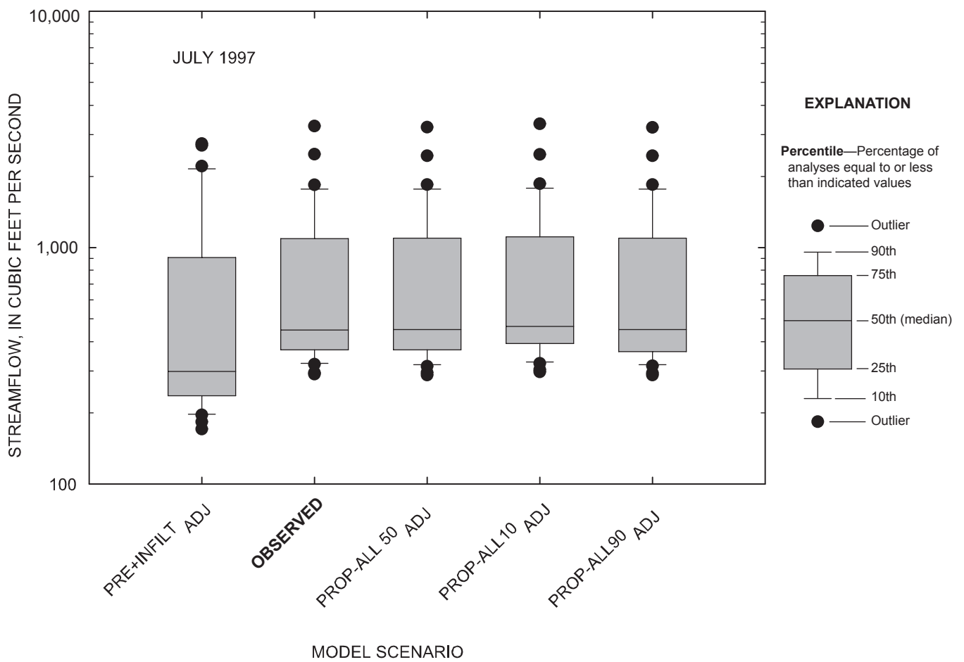
Figure 4-34. Comparison of daily streamflow for observed and simulated conditions at the Marais des Cygnes River near the Kansas-Missouri state line, Kansas, July 1997.
