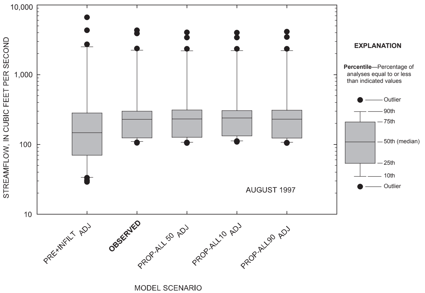
Figure 4-35. Comparison of daily streamflow for observed and simulated conditions at the Marais des Cygnes River near the Kansas-Missouri state line, Kansas, August 1997.
