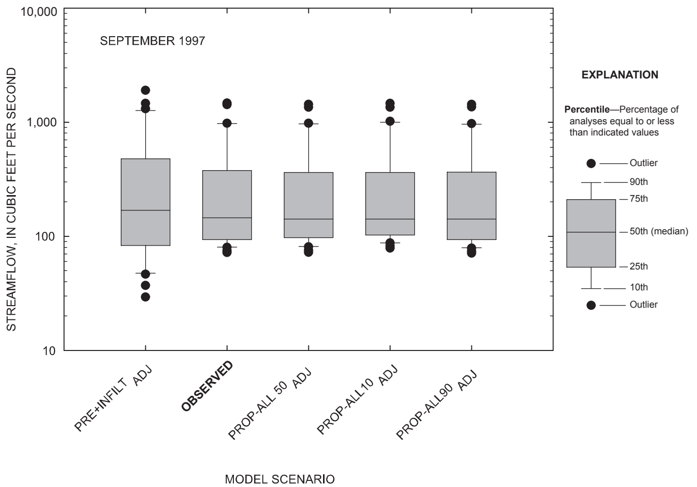
Figure 4-36. Comparison of daily streamflow for observed and simulated conditions at the Marais des Cygnes River near the Kansas-Missouri state line, Kansas, September 1997.
