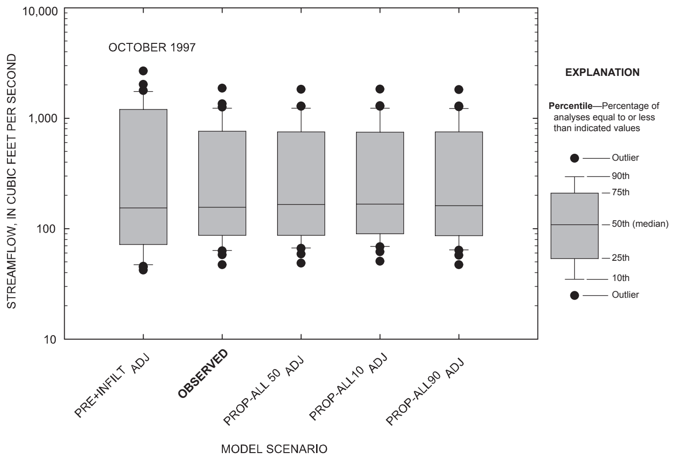
Figure 4-37. Comparison of daily streamflow for observed and simulated conditions at the Marais des Cygnes River near the Kansas-Missouri state line, Kansas, October 1997.
