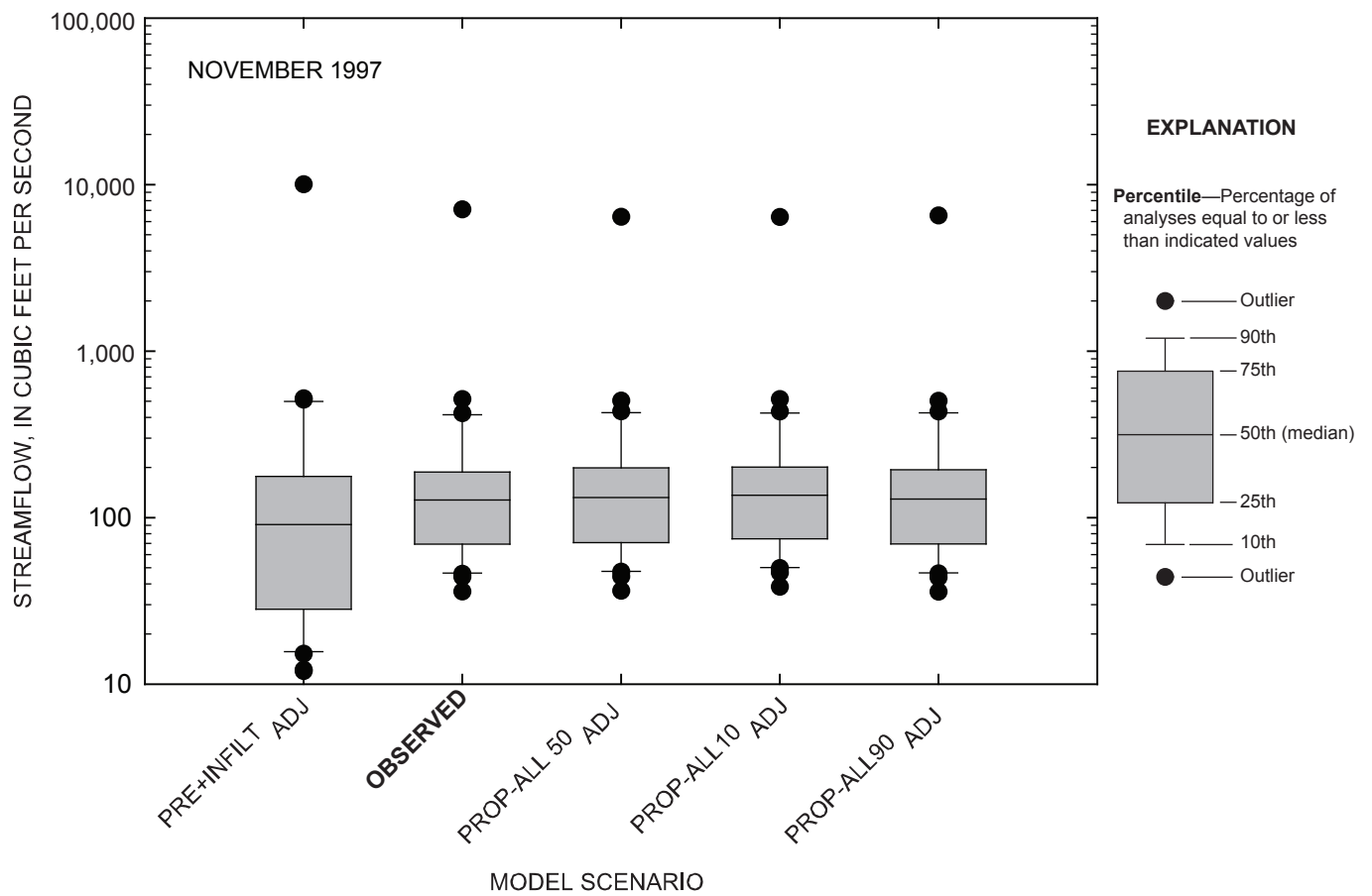
Figure 4-38. Comparison of daily streamflow for observed and simulated conditions at the Marais des Cygnes River near the Kansas-Missouri state line, Kansas, November 1997.
