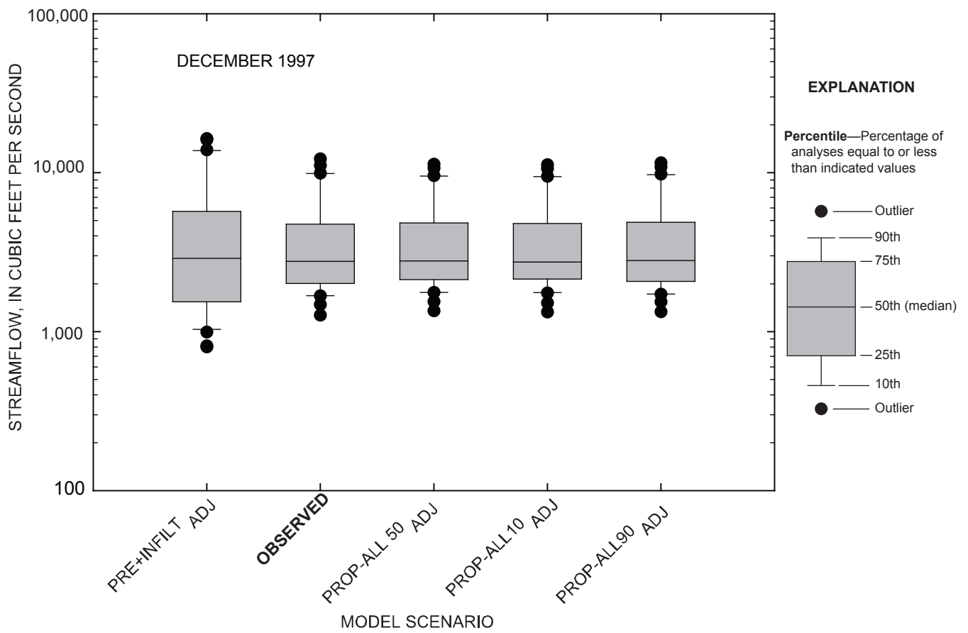
Figure 4-39. Comparison of daily streamflow for observed and simulated conditions at the Marais des Cygnes River near the Kansas-Missouri state line, Kansas, December 1997.
