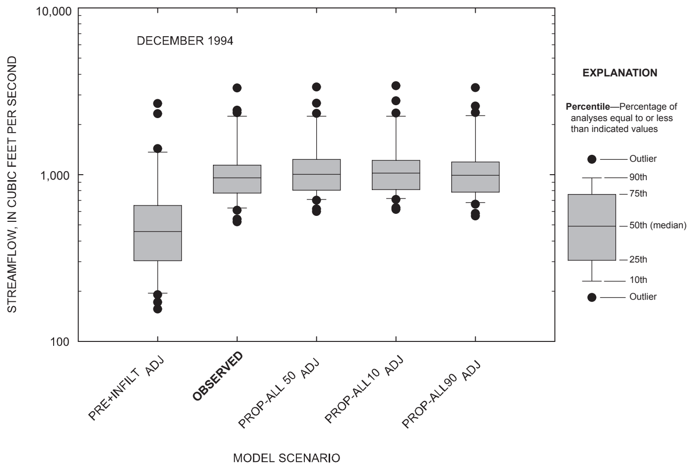
Figure 4-3. Comparison of daily streamflow for observed and simulated conditions at the Marais des Cygnes River near the Kansas-Missouri state line, Kansas, December 1994.
