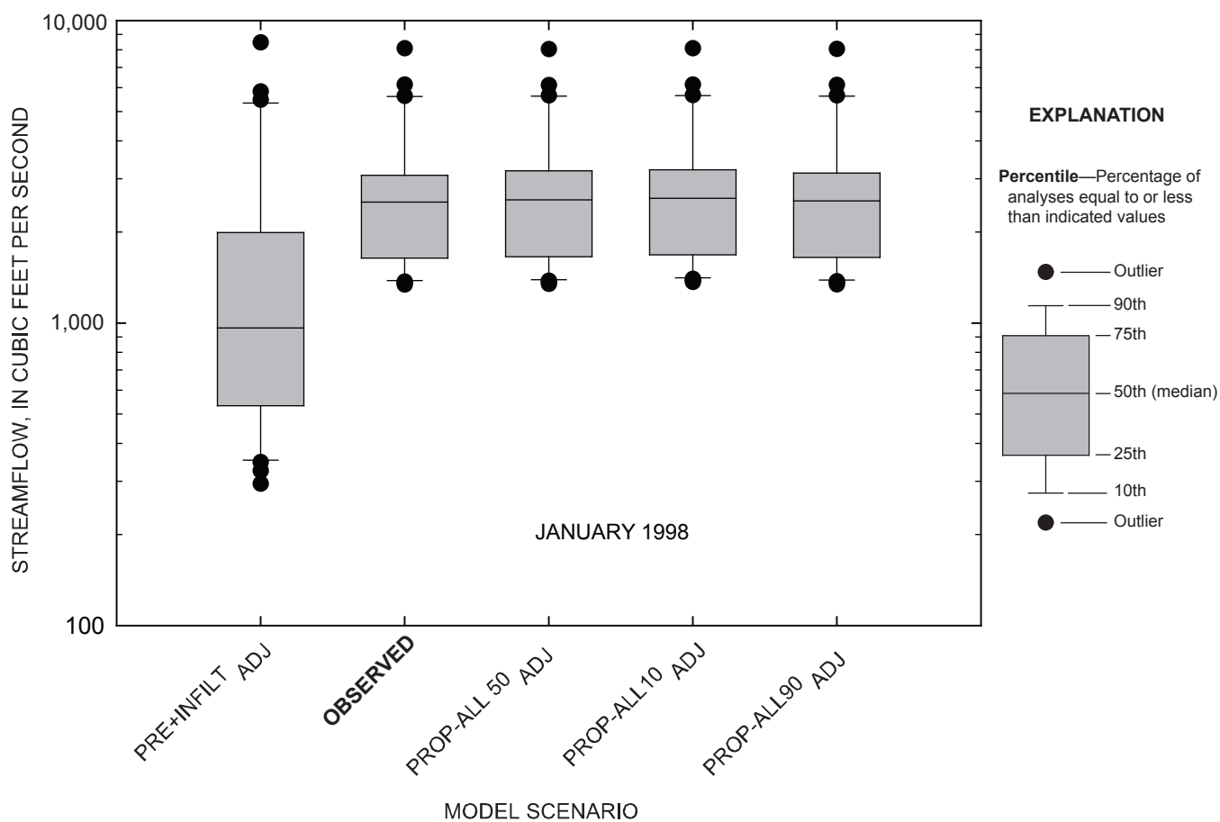
Figure 4-40. Comparison of daily streamflow for observed and simulated conditions at the Marais des Cygnes River near the Kansas-Missouri state line, Kansas, January 1998.
