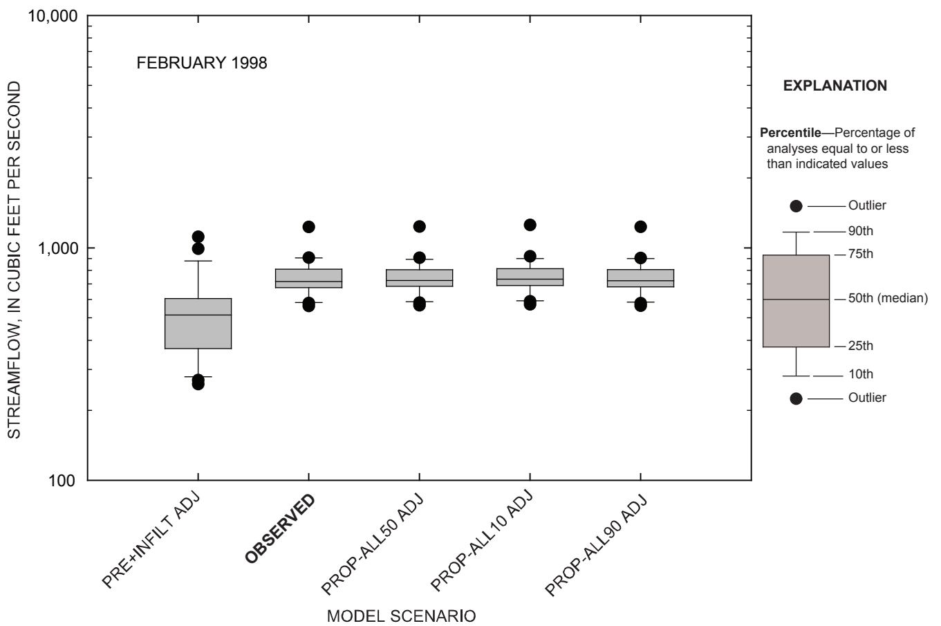
Figure 4-41. Comparison of daily streamflow for observed and simulated conditions at the Marais des Cygnes River near the Kansas-Missouri state line, Kansas, February 1998.
