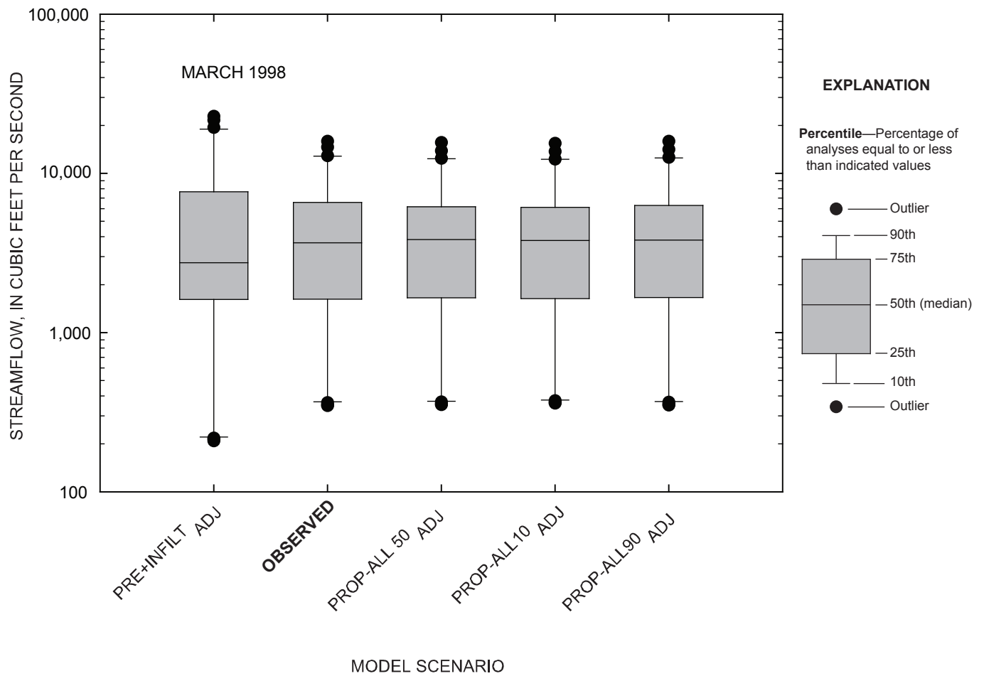
Figure 4-42. Comparison of daily streamflow for observed and simulated conditions at the Marais des Cygnes River near the Kansas-Missouri state line, Kansas, March 1998.
