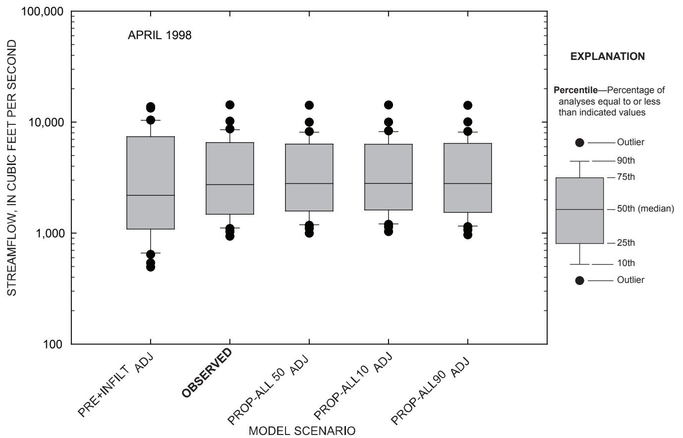
Figure 4-43. Comparison of daily streamflow for observed and simulated conditions at the Marais des Cygnes River near the Kansas-Missouri state line, Kansas, April 1998.
