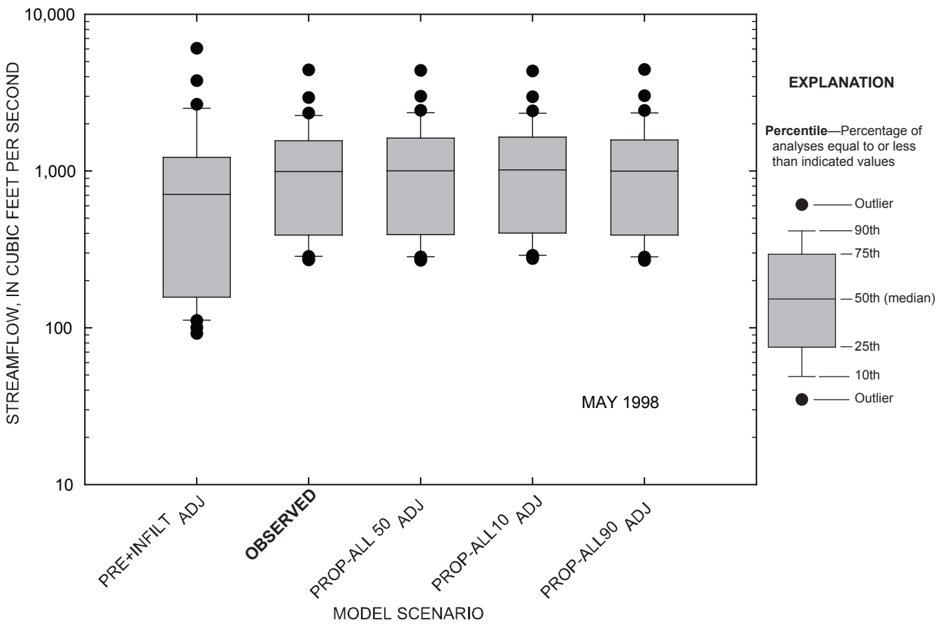
Figure 4-44. Comparison of daily streamflow for observed and simulated conditions at the Marais des Cygnes River near the Kansas-Missouri state line, Kansas, May 1998.
