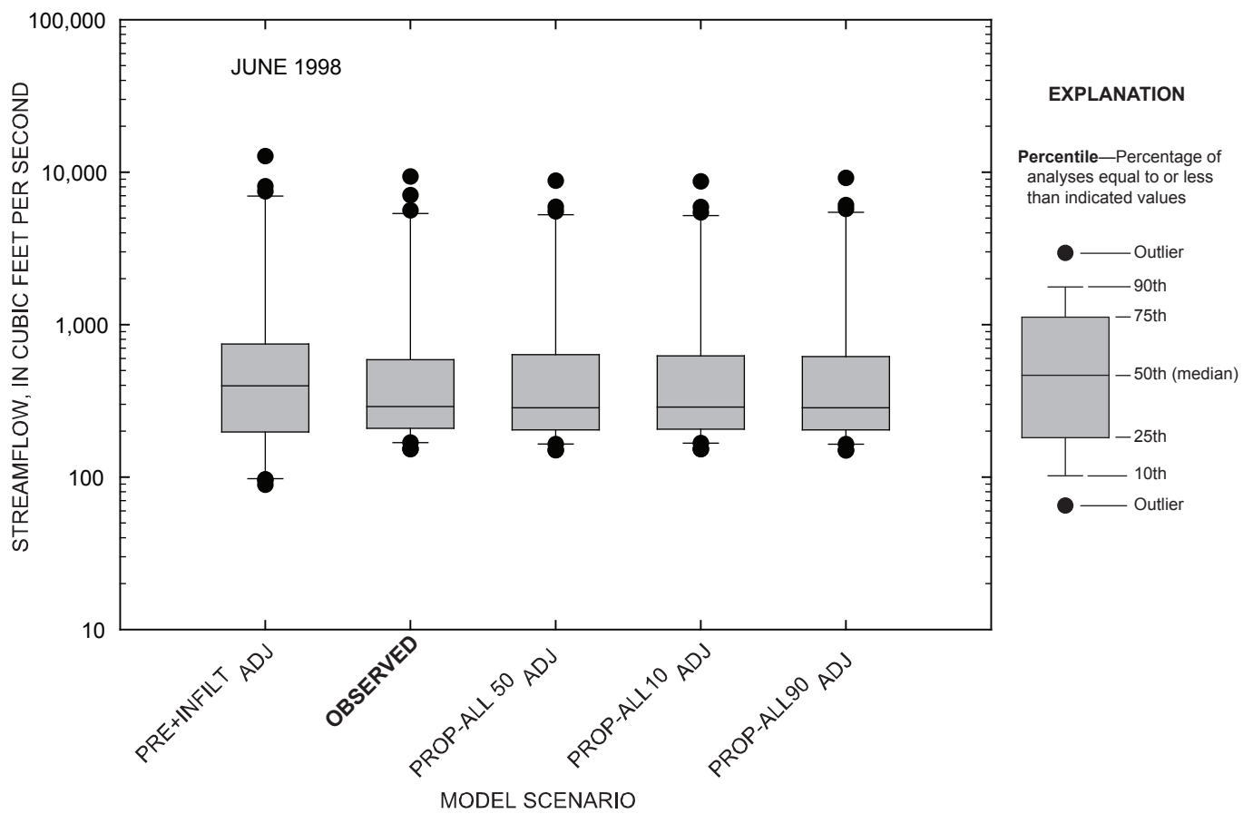
Figure 4-45. Comparison of daily streamflow for observed and simulated conditions at the Marais des Cygnes River near the Kansas-Missouri state line, Kansas, June 1998.
