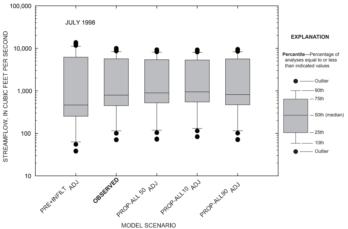
Figure 4-46. Comparison of daily streamflow for observed and simulated conditions at the Marais des Cygnes River near the Kansas-Missouri state line, Kansas, July 1998.
