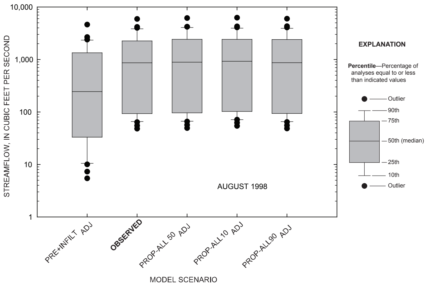
Figure 4-47. Comparison of daily streamflow for observed and simulated conditions at the Marais des Cygnes River near the Kansas-Missouri state line, Kansas, August 1998.
