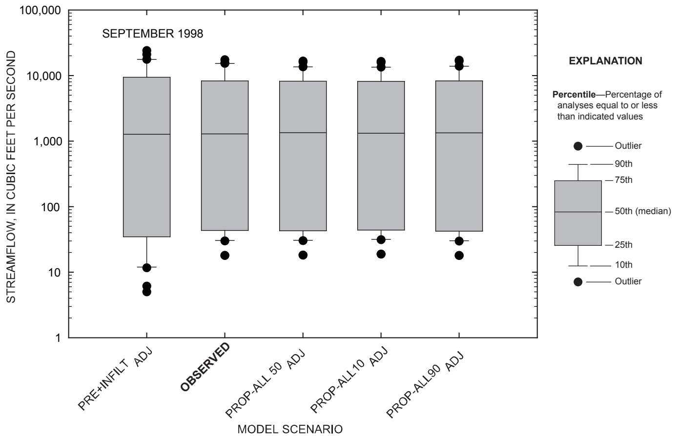
Figure 4-48. Comparison of daily streamflow for observed and simulated conditions at the Marais des Cygnes River near the Kansas-Missouri state line, Kansas, September 1998.
