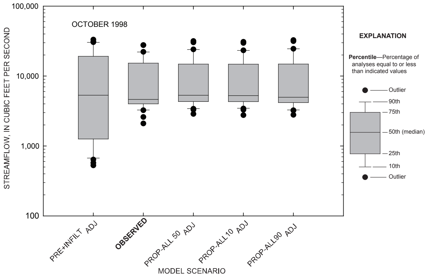
Figure 4-49. Comparison of daily streamflow for observed and simulated conditions at the Marais des Cygnes River near the Kansas-Missouri state line, Kansas, October 1998.
