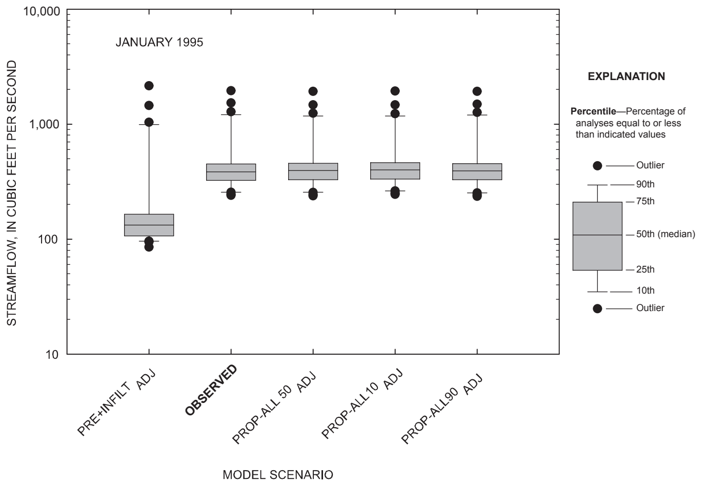
Figure 4-4. Comparison of daily streamflow for observed and simulated conditions at the Marais des Cygnes River near the Kansas-Missouri state line, Kansas, January 1995.
