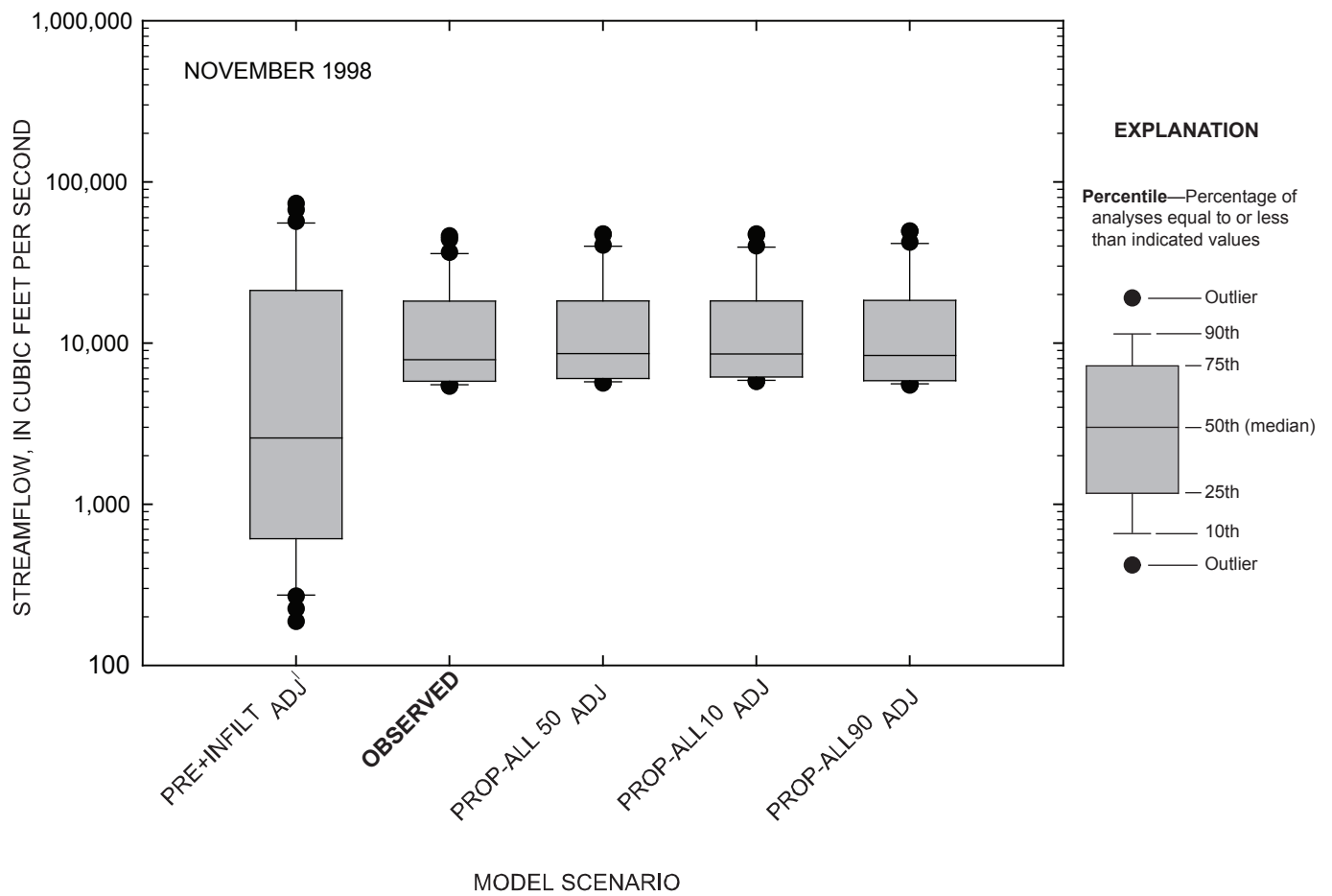
Figure 4-50. Comparison of daily streamflow for observed and simulated conditions at the Marais des Cygnes River near the Kansas-Missouri state line, Kansas, November 1998.
