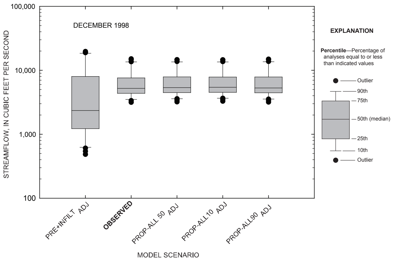
Figure 4-51. Comparison of daily streamflow for observed and simulated conditions at the Marais des Cygnes River near the Kansas-Missouri state line, Kansas, December 1998.
