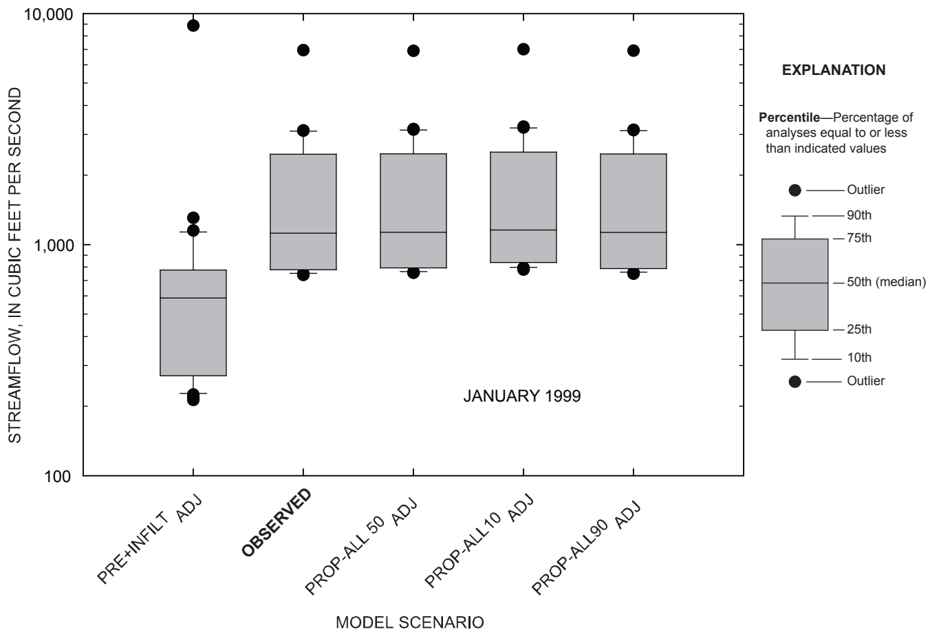
Figure 4-52. Comparison of daily streamflow for observed and simulated conditions at the Marais des Cygnes River near the Kansas-Missouri state line, Kansas, January 1999.
