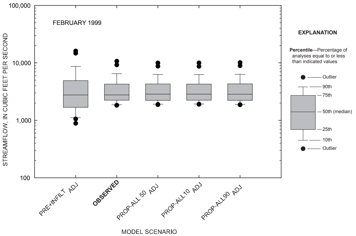
Figure 4-53. Comparison of daily streamflow for observed and simulated conditions at the Marais des Cygnes River near the Kansas-Missouri state line, Kansas, February 1999.
