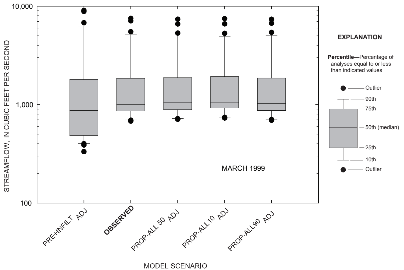
Figure 4-54. Comparison of daily streamflow for observed and simulated conditions at the Marais des Cygnes River near the Kansas-Missouri state line, Kansas, March 1999.
