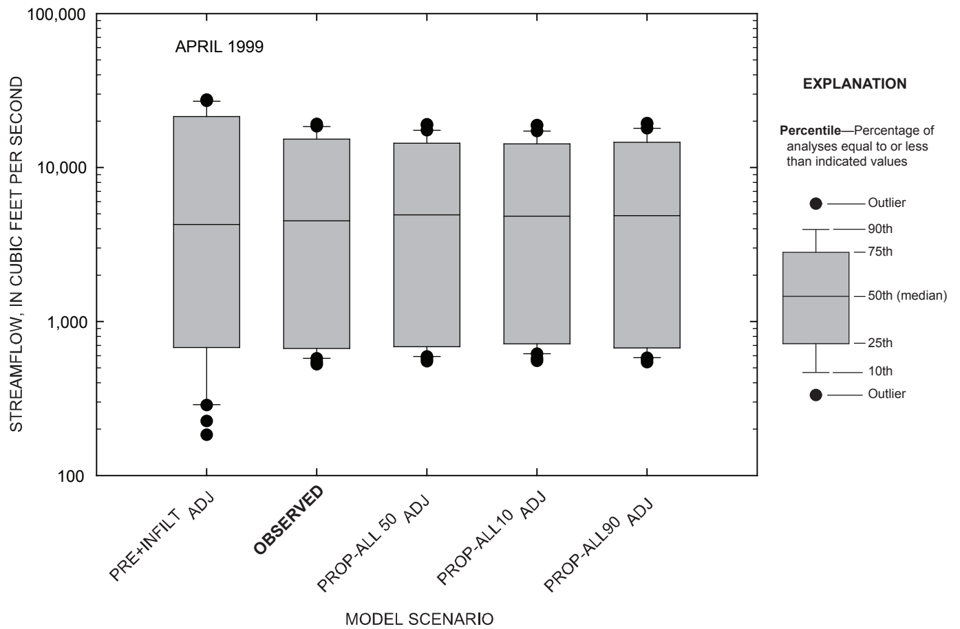
Figure 4-55. Comparison of daily streamflow for observed and simulated conditions at the Marais des Cygnes River near the Kansas-Missouri state line, Kansas, April 1999.
