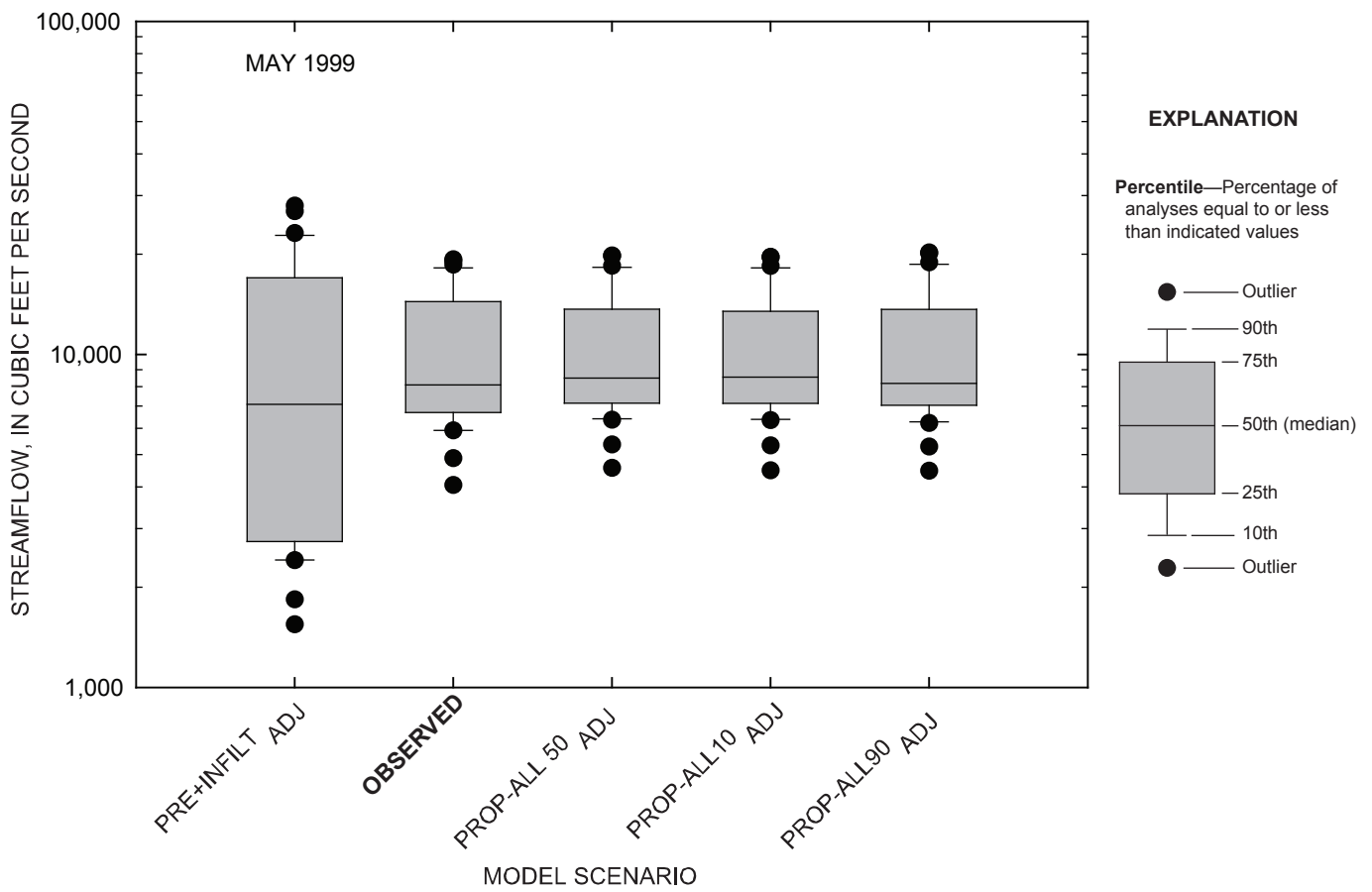
Figure 4-56. Comparison of daily streamflow for observed and simulated conditions at the Marais des Cygnes River near the Kansas-Missouri state line, Kansas, May 1999.
