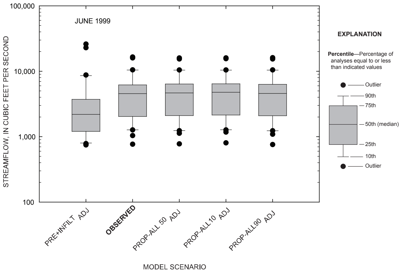
Figure 4-57. Comparison of daily streamflow for observed and simulated conditions at the Marais des Cygnes River near the Kansas-Missouri state line, Kansas, June 1999.
