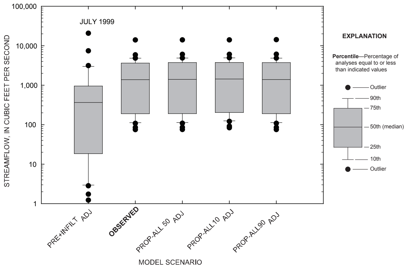
Figure 4-58. Comparison of daily streamflow for observed and simulated conditions at the Marais des Cygnes River near the Kansas-Missouri state line, Kansas, July 1999.
