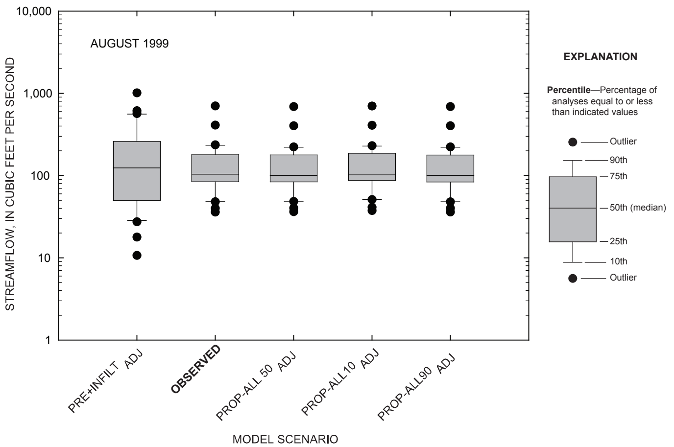
Figure 4-59. Comparison of daily streamflow for observed and simulated conditions at the Marais des Cygnes River near the Kansas-Missouri state line, Kansas, August 1999.
