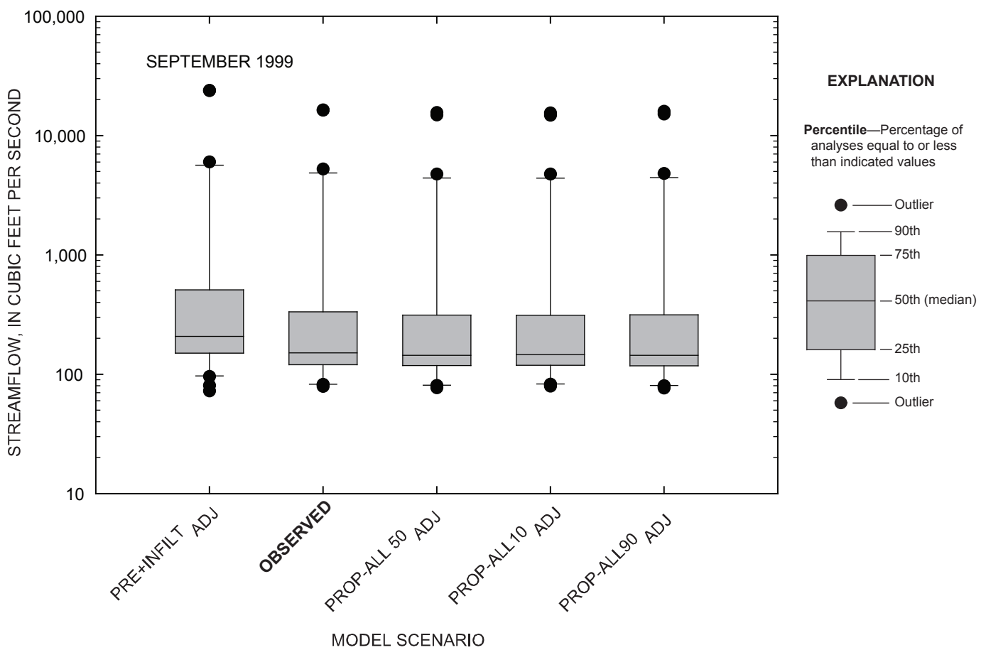
Figure 4-60. Comparison of daily streamflow for observed and simulated conditions at the Marais des Cygnes River near the Kansas-Missouri state line, Kansas, September 1999.
