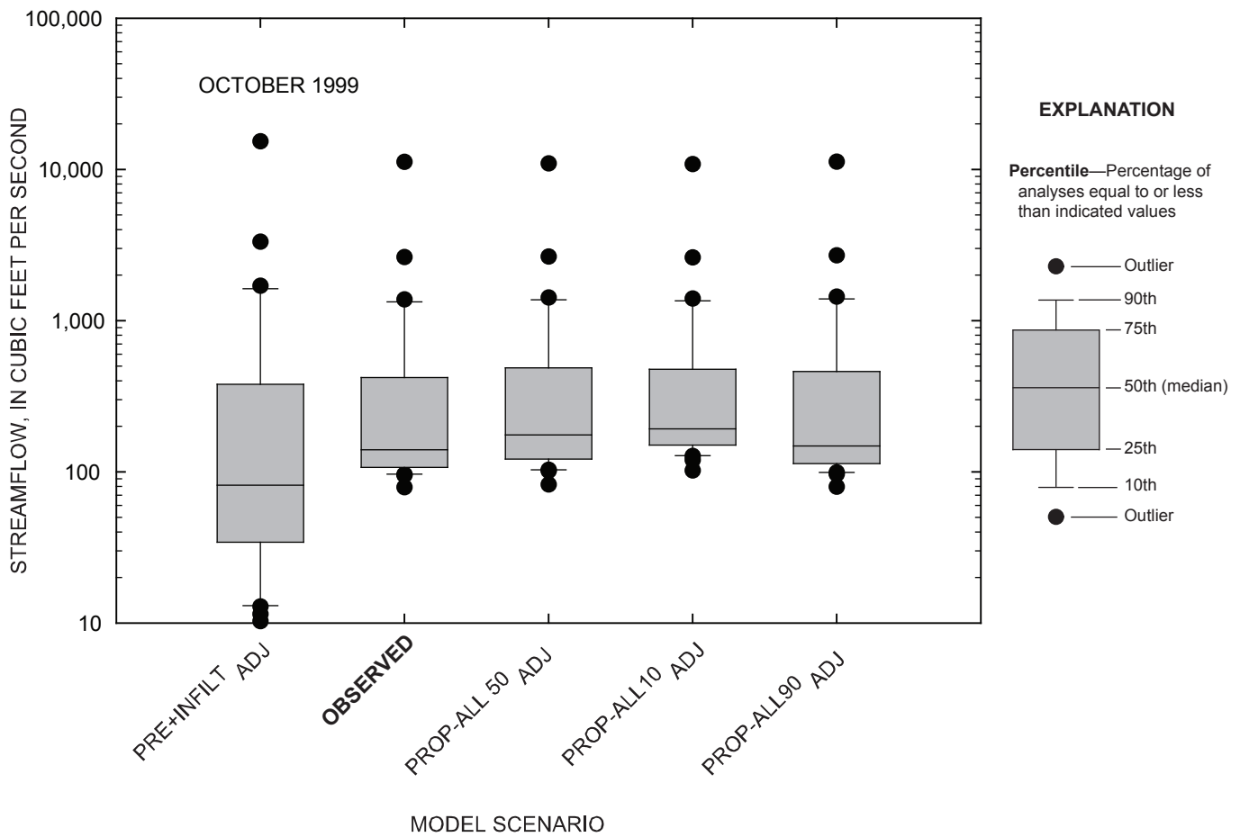
Figure 4-61. Comparison of daily streamflow for observed and simulated conditions at the Marais des Cygnes River near the Kansas-Missouri state line, Kansas, October 1999.
