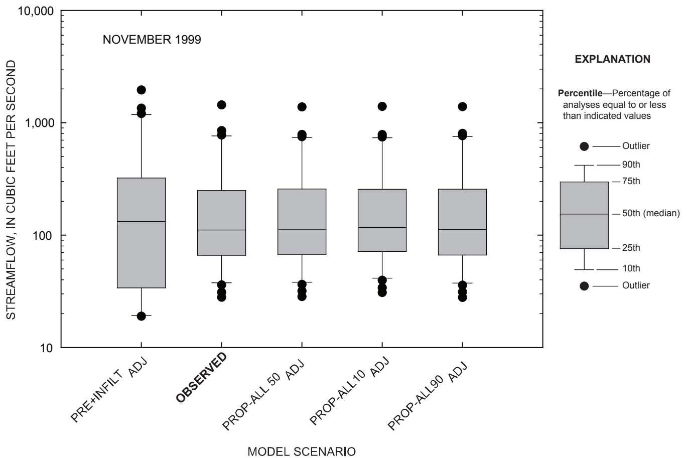
Figure 4-62. Comparison of daily streamflow for observed and simulated conditions at the Marais des Cygnes River near the Kansas-Missouri state line, Kansas, November 1999.
