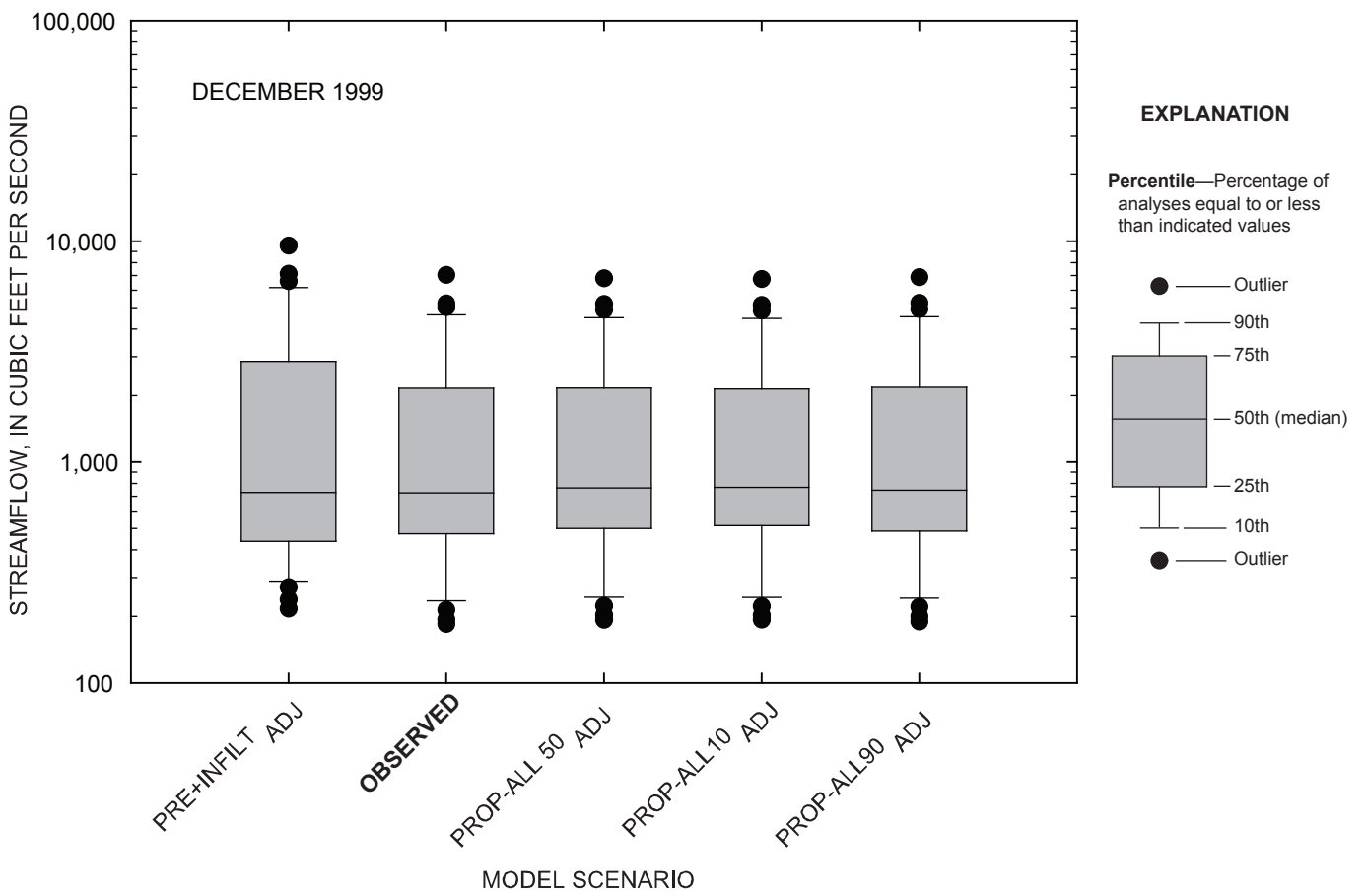
Figure 4-63. Comparison of daily streamflow for observed and simulated conditions at the Marais des Cygnes River near the Kansas-Missouri state line, Kansas, December 1999.
