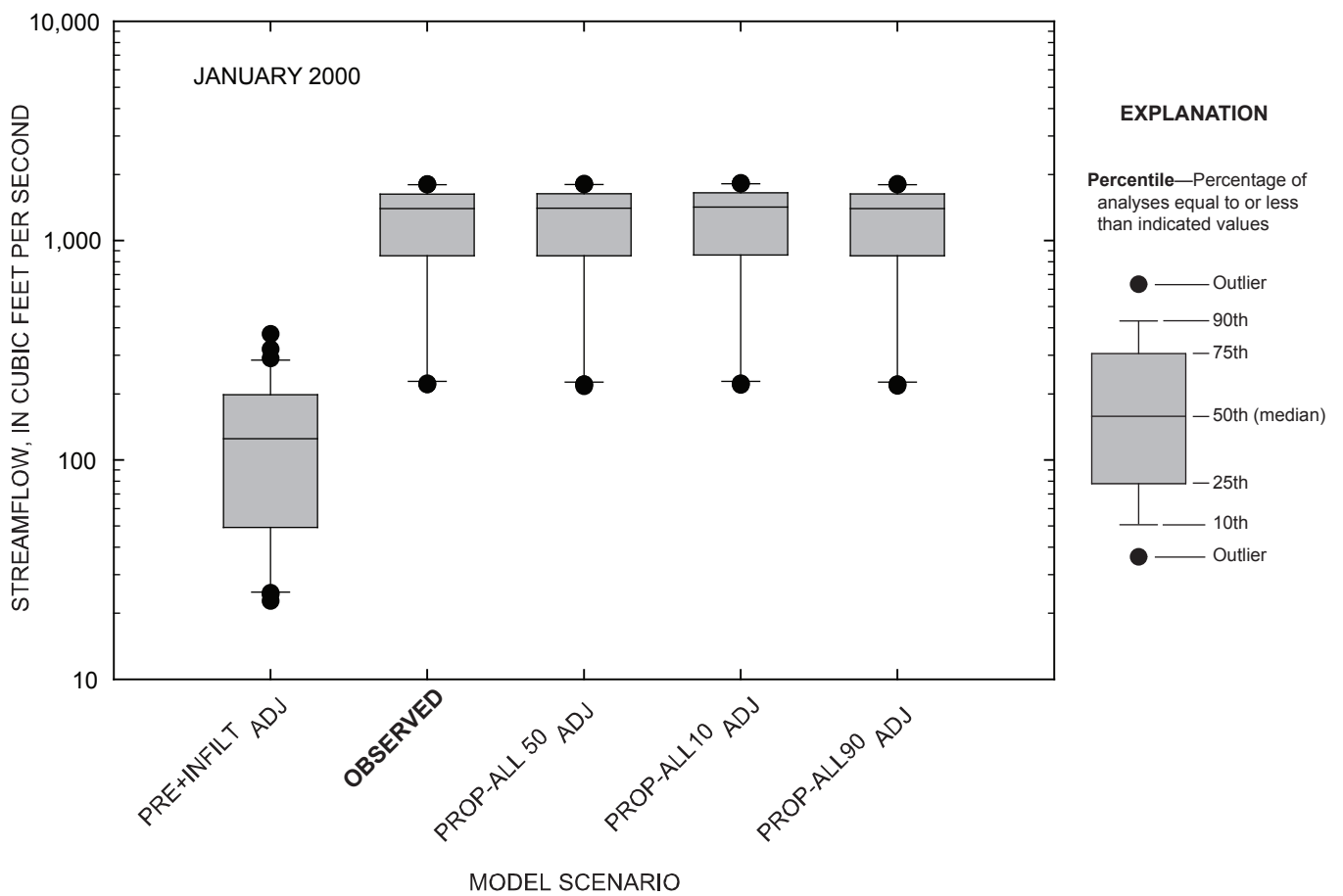
Figure 4-64. Comparison of daily streamflow for observed and simulated conditions at the Marais des Cygnes River near the Kansas-Missouri state line, Kansas, January 2000.
