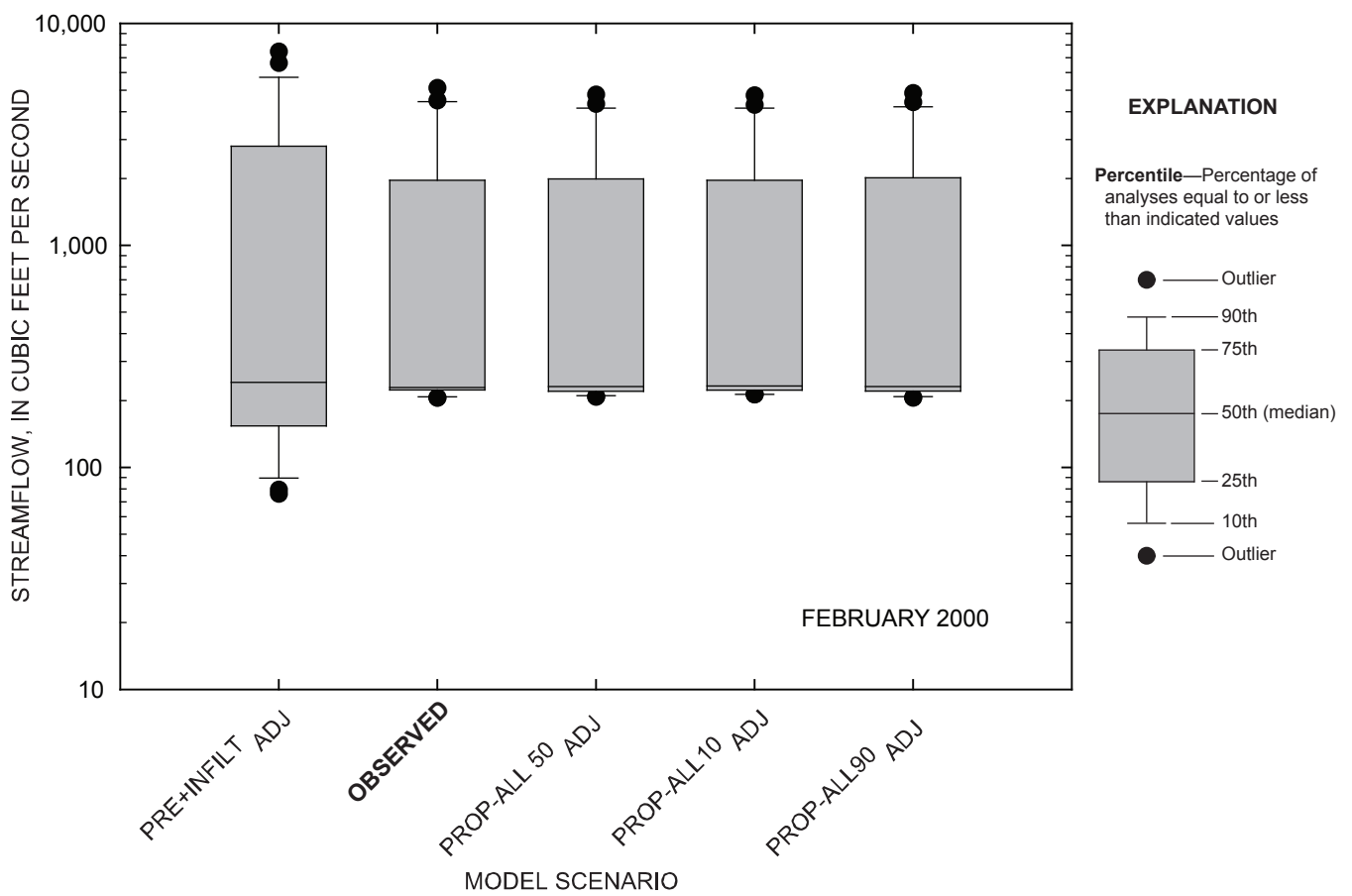
Figure 4-65. Comparison of daily streamflow for observed and simulated conditions at the Marais des Cygnes River near the Kansas-Missouri state line, Kansas, February 2000.
