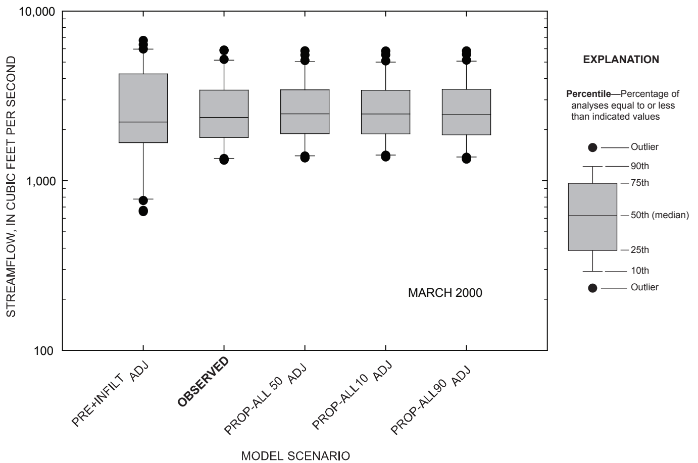
Figure 4-66. Comparison of daily streamflow for observed and simulated conditions at the Marais des Cygnes River near the Kansas-Missouri state line, Kansas, March 2000.
