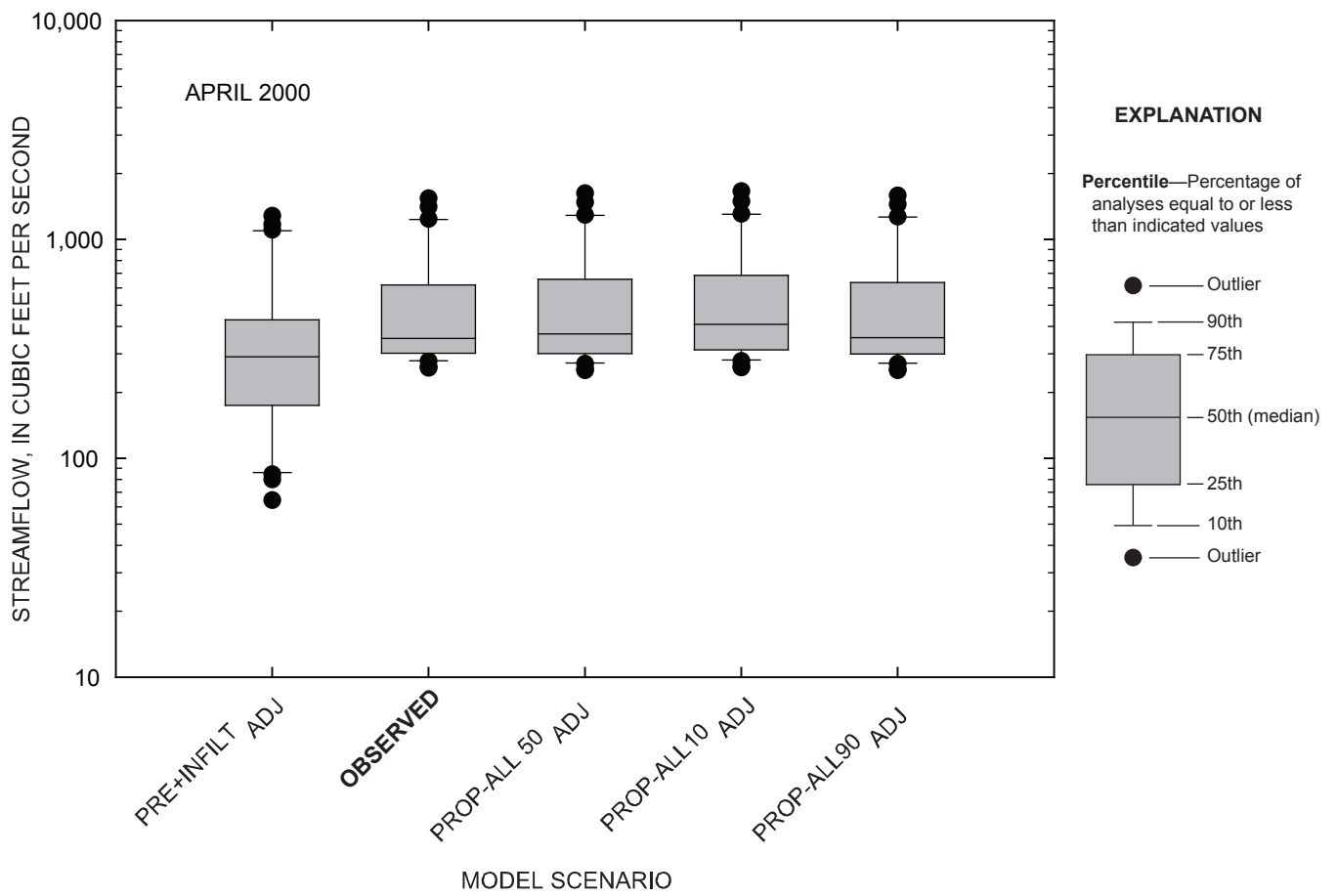
Figure 4-67. Comparison of daily streamflow for observed and simulated conditions at the Marais des Cygnes River near the Kansas-Missouri state line, Kansas, April 2000.
