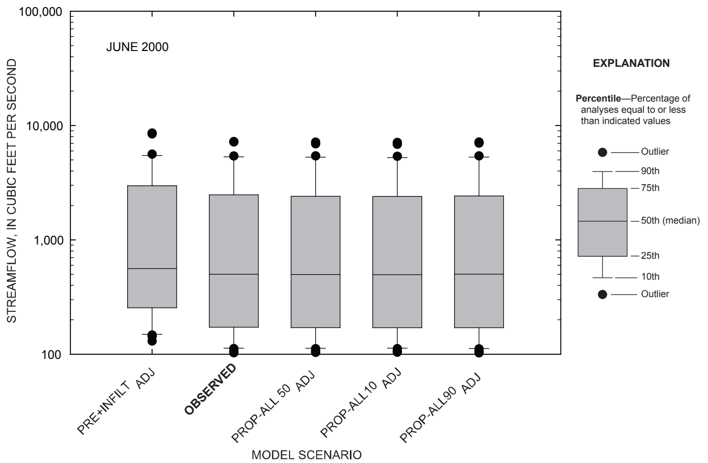
Figure 4-69. Comparison of daily streamflow for observed and simulated conditions at the Marais des Cygnes River near the Kansas-Missouri state line, Kansas, June 2000.
