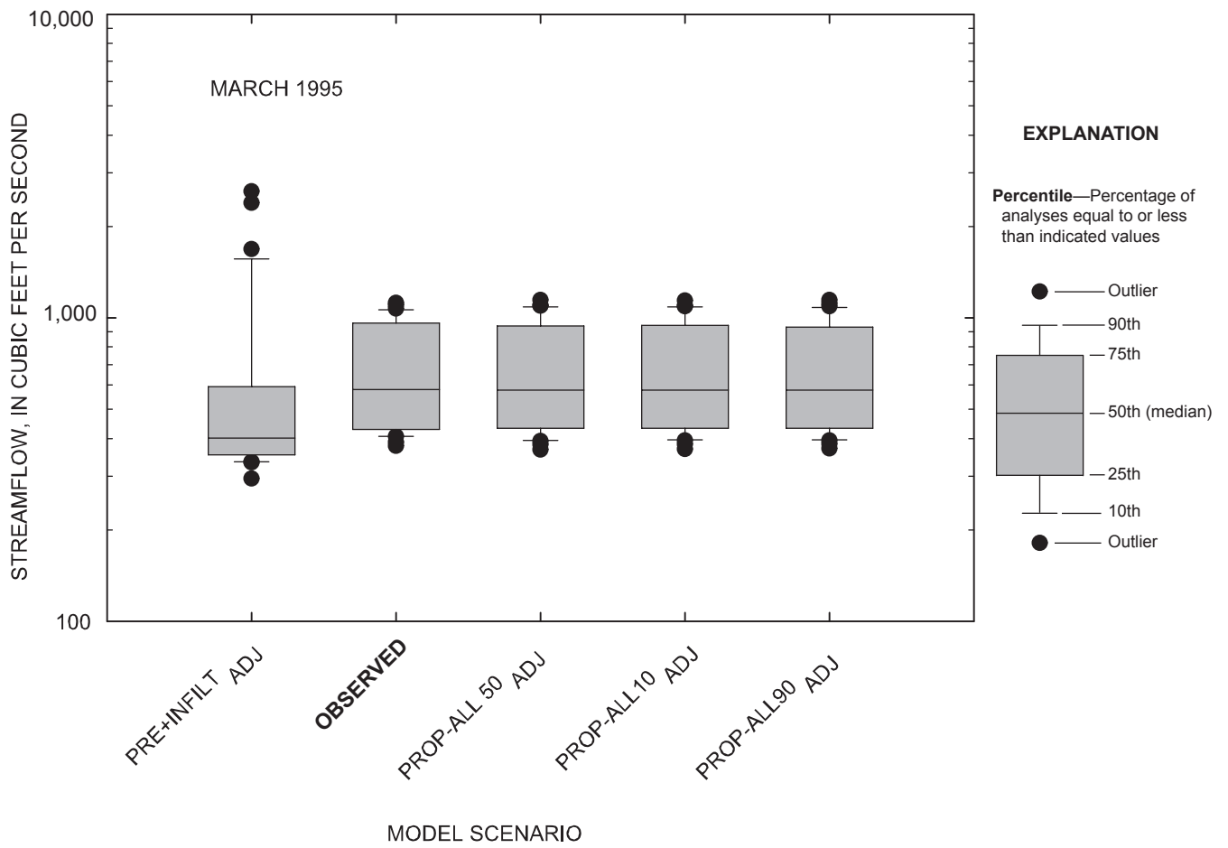
Figure 4-6. Comparison of daily streamflow for observed and simulated conditions at the Marais des Cygnes River near the Kansas-Missouri state line, Kansas, March 1995.
