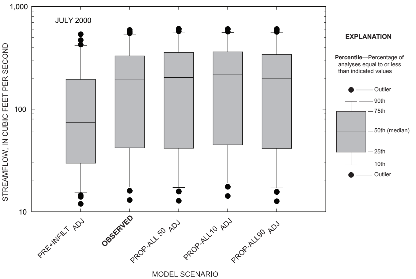
Figure 4-70. Comparison of daily streamflow for observed and simulated conditions at the Marais des Cygnes River near the Kansas-Missouri state line, Kansas, July 2000.
