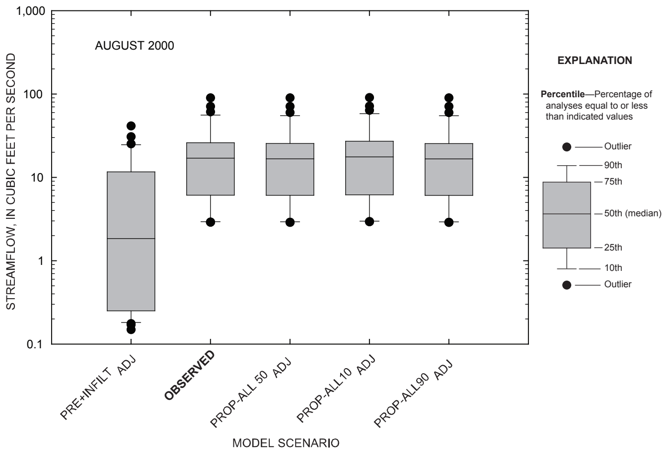
Figure 4-71. Comparison of daily streamflow for observed and simulated conditions at the Marais des Cygnes River near the Kansas-Missouri state line, Kansas, August 2000.
