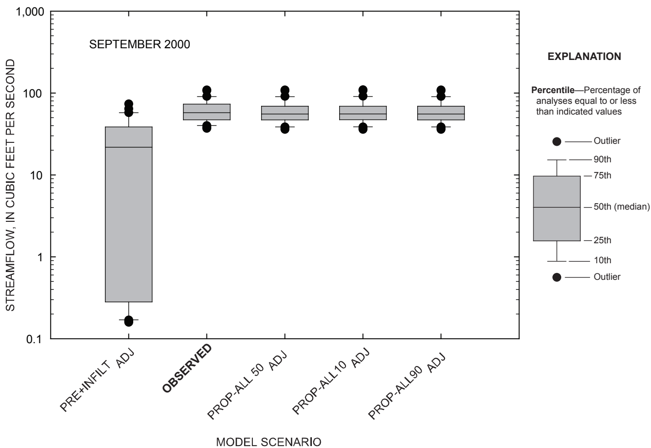
Figure 4-72. Comparison of daily streamflow for observed and simulated conditions at the Marais des Cygnes River near the Kansas-Missouri state line, Kansas, September 2000.
