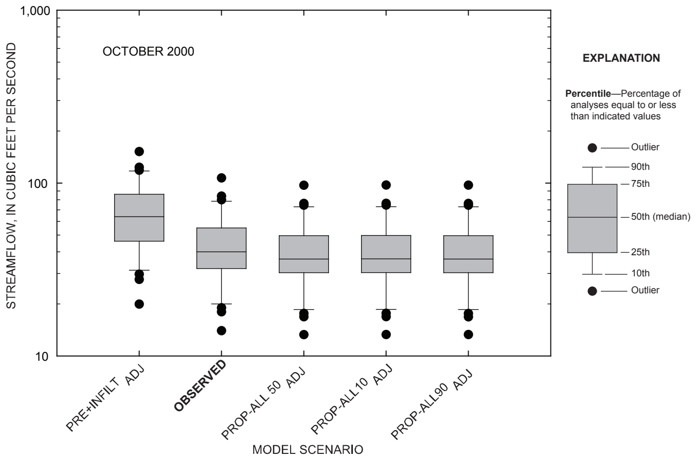
Figure 4-73. Comparison of daily streamflow for observed and simulated conditions at the Marais des Cygnes River near the Kansas-Missouri state line, Kansas, October 2000.
