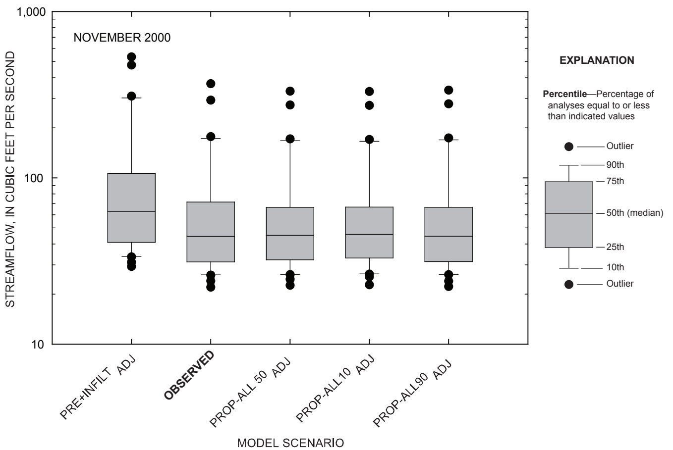
Figure 4-74. Comparison of daily streamflow for observed and simulated conditions at the Marais des Cygnes River near the Kansas-Missouri state line, Kansas, November 2000.
