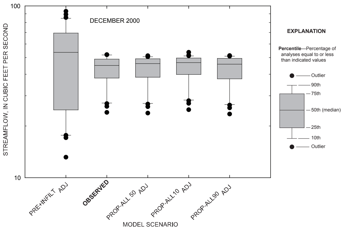
Figure 4-75. Comparison of daily streamflow for observed and simulated conditions at the Marais des Cygnes River near the Kansas-Missouri state line, Kansas, December 2000.
