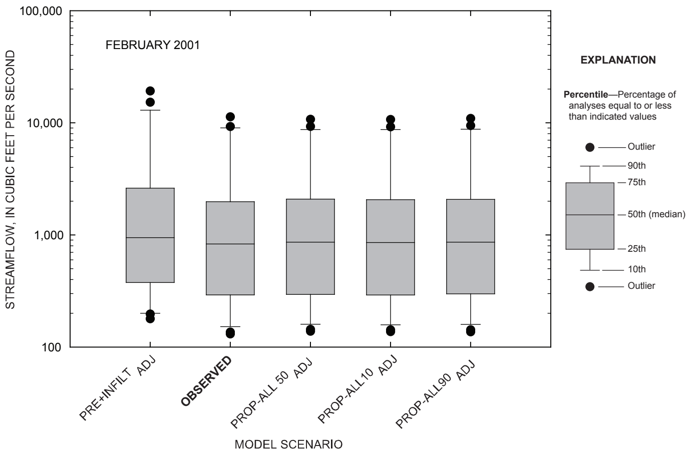
Figure 4-77. Comparison of daily streamflow for observed and simulated conditions at the Marais des Cygnes River near the Kansas-Missouri state line, Kansas, February 2001.
