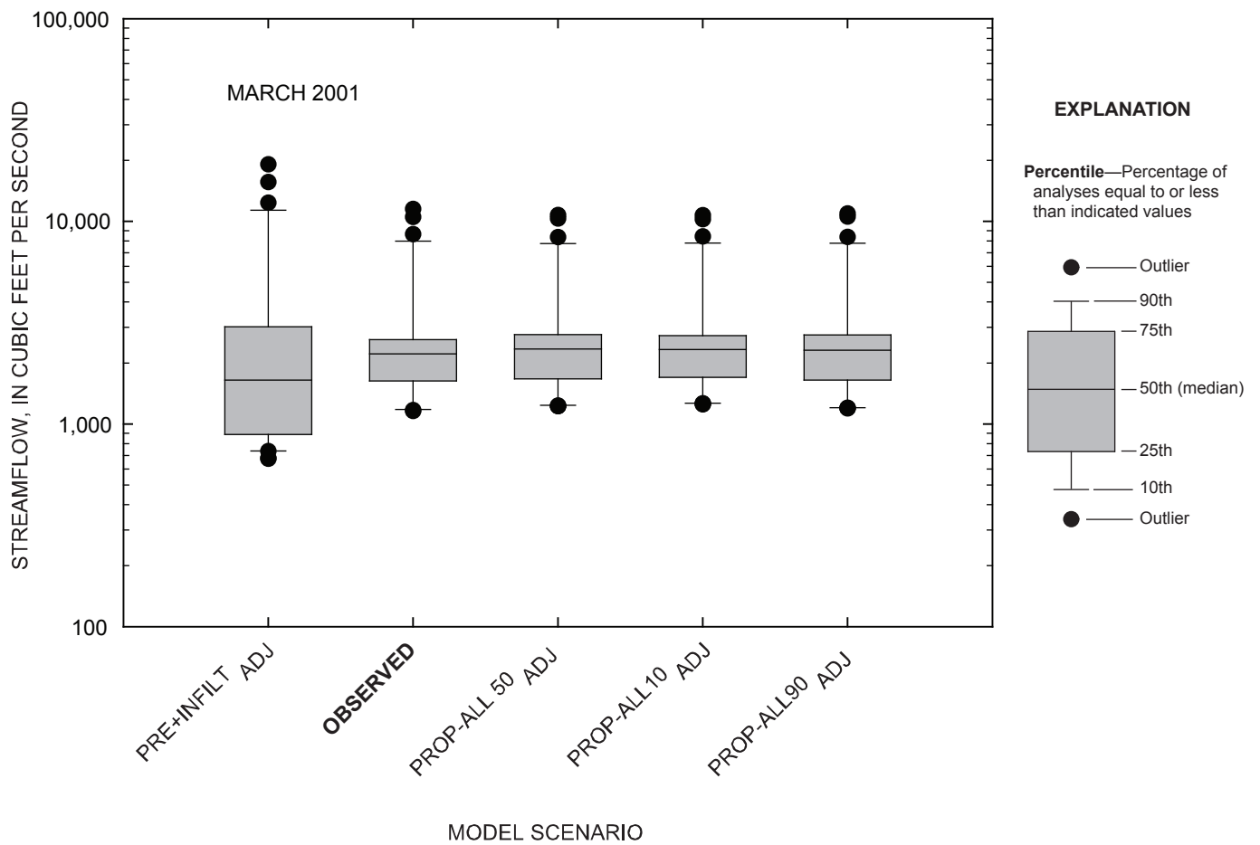
Figure 4-78. Comparison of daily streamflow for observed and simulated conditions at the Marais des Cygnes River near the Kansas-Missouri state line, Kansas, March 2001.
