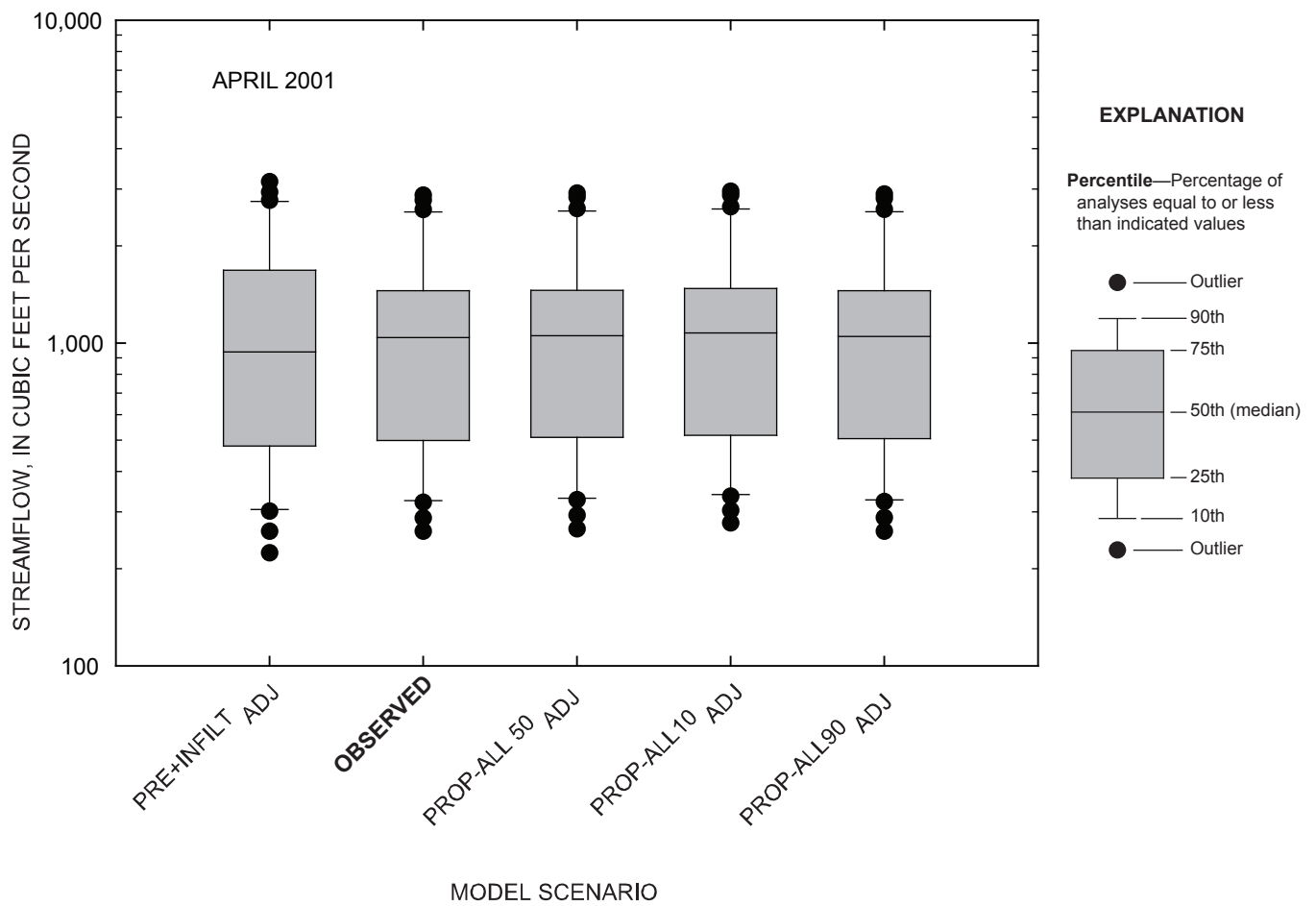
Figure 4-79. Comparison of daily streamflow for observed and simulated conditions at the Marais des Cygnes River near the Kansas-Missouri state line, Kansas, April 2001.
