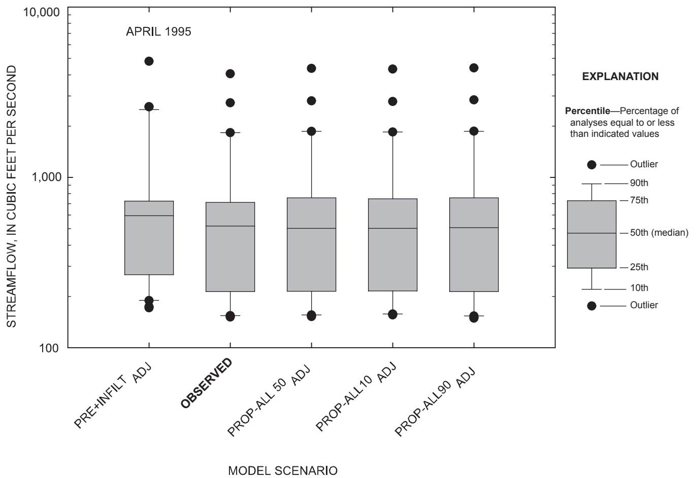
Figure 4-7. Comparison of daily streamflow for observed and simulated conditions at the Marais des Cygnes River near the Kansas-Missouri state line, Kansas, April 1995.
