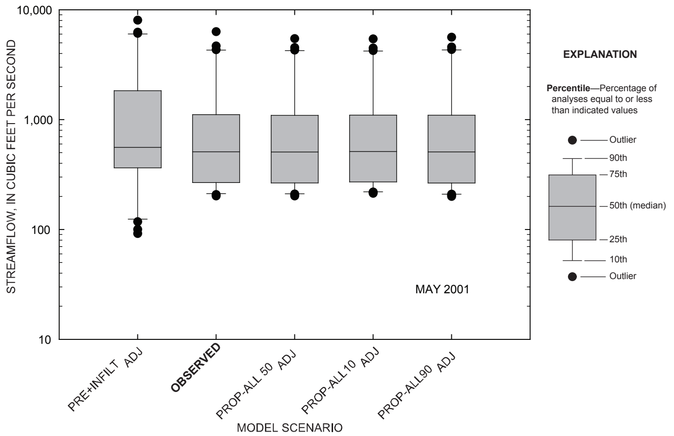
Figure 4-80. Comparison of daily streamflow for observed and simulated conditions at the Marais des Cygnes River near the Kansas-Missouri state line, Kansas, May 2001.
